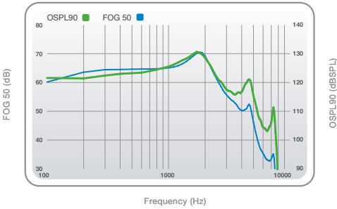
OSPL90 (green) and Full-On Gain (blue) curves for the Focus CIC at the highest matrix of 130/70.
