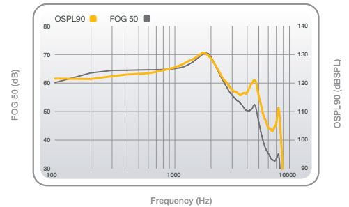
OSPL90 (yellow) and Full-On Gain (gray) curves for the Avail CIC at the highest matrix of 130/70.
